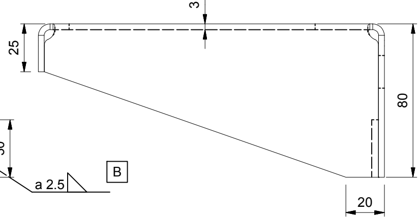
Side view ( 1 : 2 )
