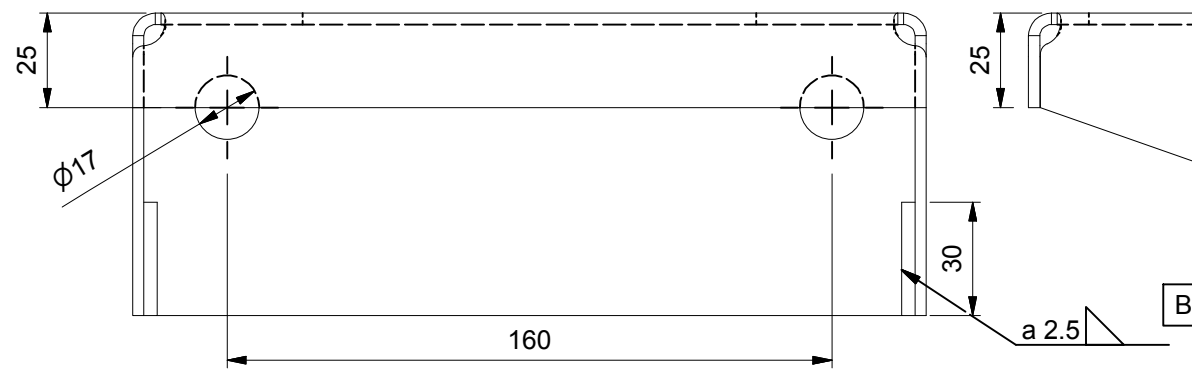
Front view ( 1 : 2 )
