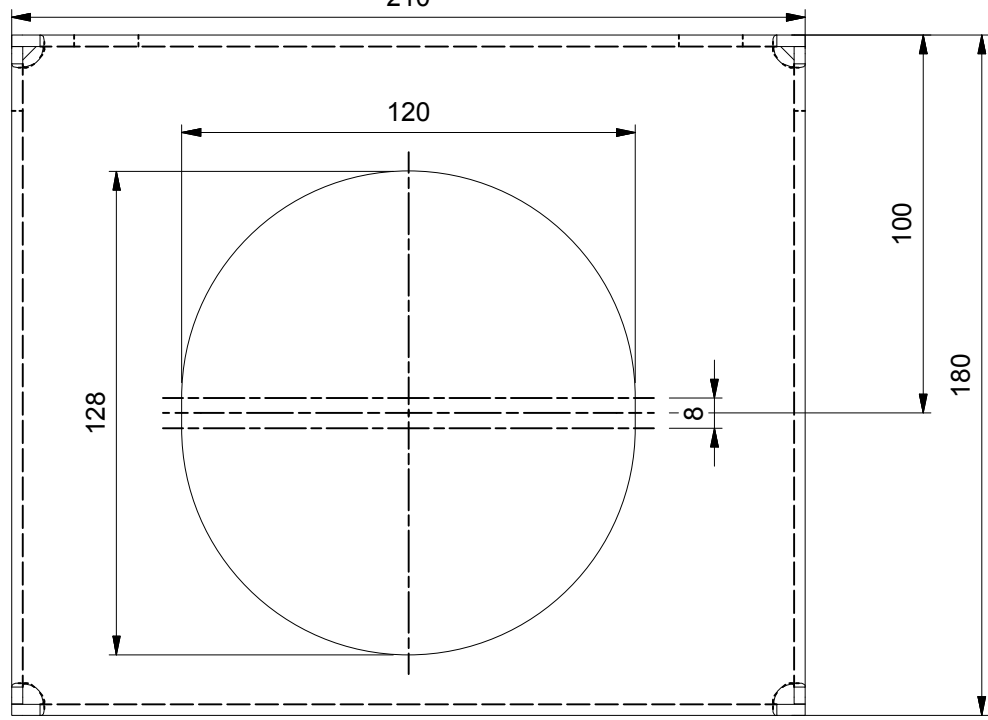
Front view ( 1 : 2 )
