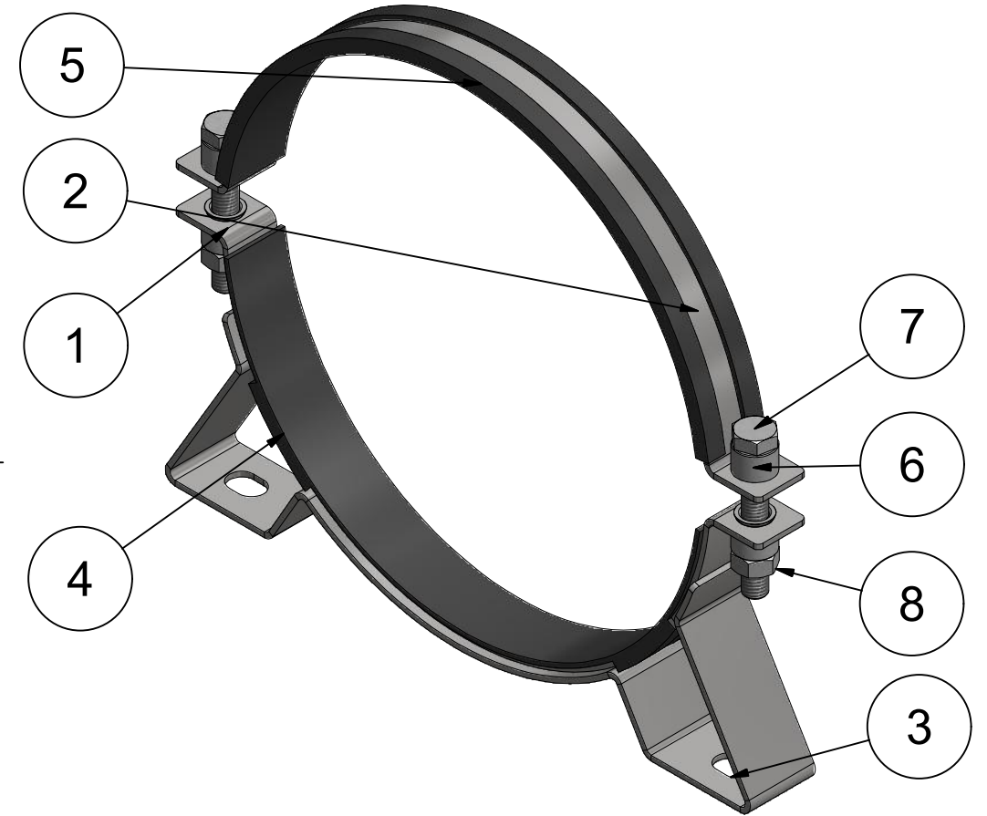
Parts identification ( 1 : 3 )
