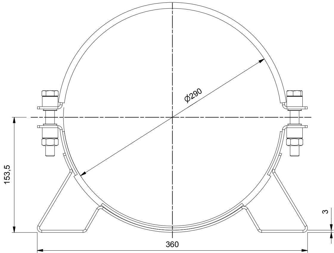
Front view ( 1 : 3 )
