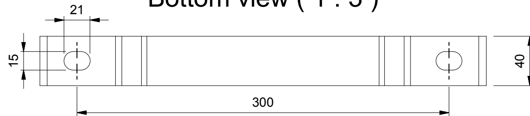
Bottom view ( 1 : 3 )
