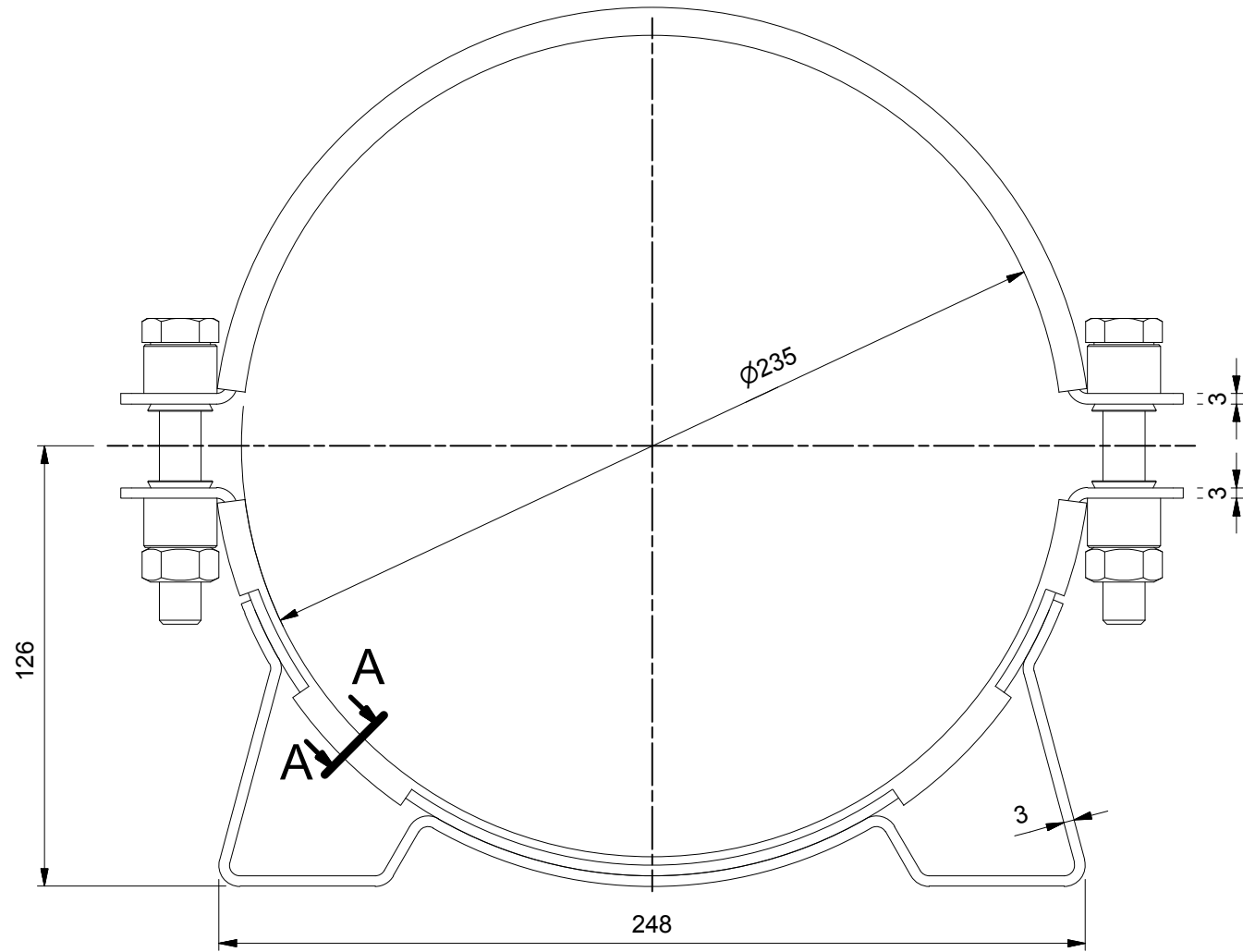
Bottom view ( 1 : 2 )
