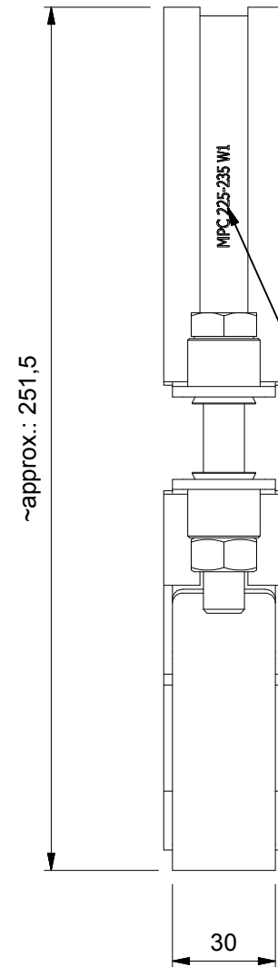
Side view ( 1 : 2 )
